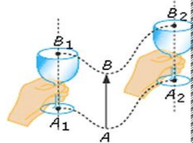
Translation curviligne
